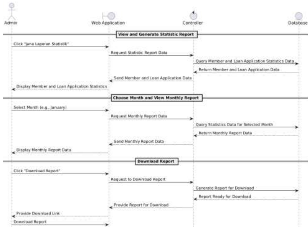
Figure 4.4.11: SD011 Sequence Diagram for < Admin view administrative report >
